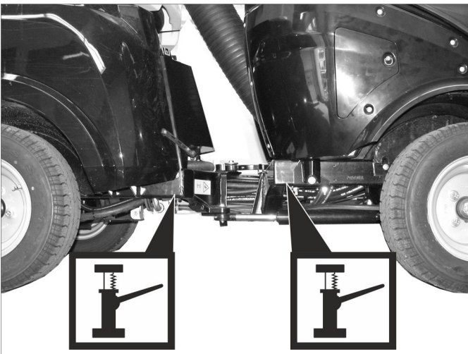
Intake points for the jack
